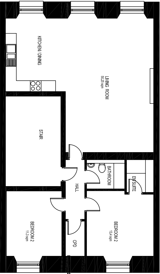
FLAT 2 WOODSIDE PLACE GLASGOW G3 7QF FIRST FLOOR - GROSS INTERNAL AREA = 93m 2 (1001 SQ. FT.)
